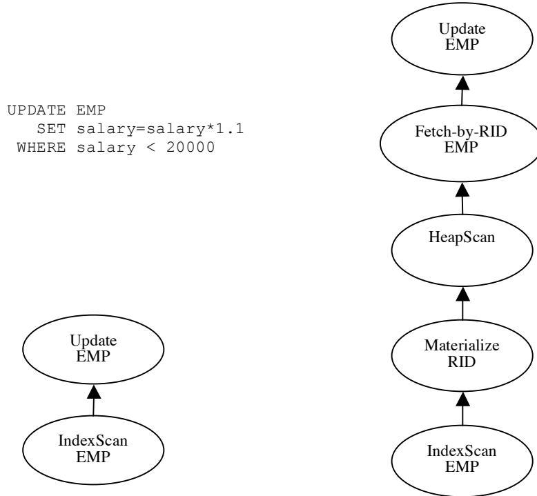
Figure 10: Two query plans for updating a table via an IndexScan. The plan on the left is susceptible to the Halloween problem. The plan on the right is safe, since it identifies all tuples to be updated before doing any updates.
